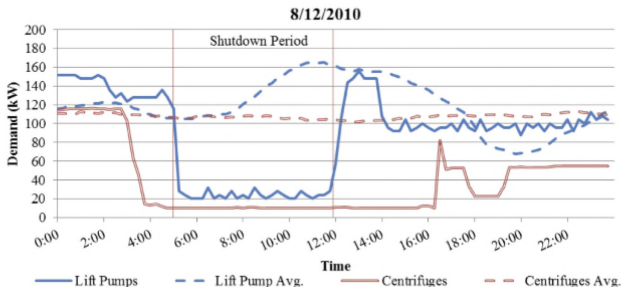
Figure 14: Reductions in lift pump and centrifuge demand during a partial-day plant shutdown.
